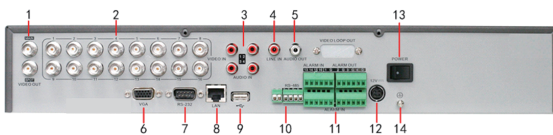
Rear Panel of DS-7216HVI-ST
